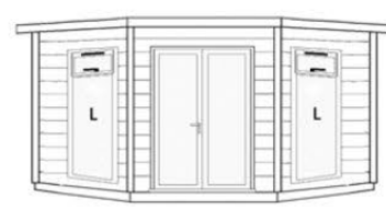
9' (2.74m) front with French full length double doors & 2 (L) 1180mm opening windows to front
