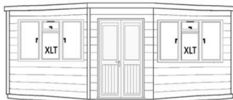
11' (3.35m) front with French 1/2 length double doors & 2 (XLT) 1800mm opening windows to front
